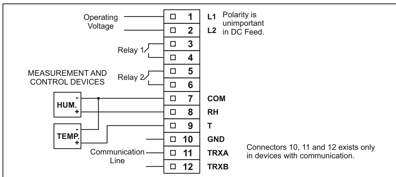
Figure 5.1. Connection Diagram of E-RHT-20
